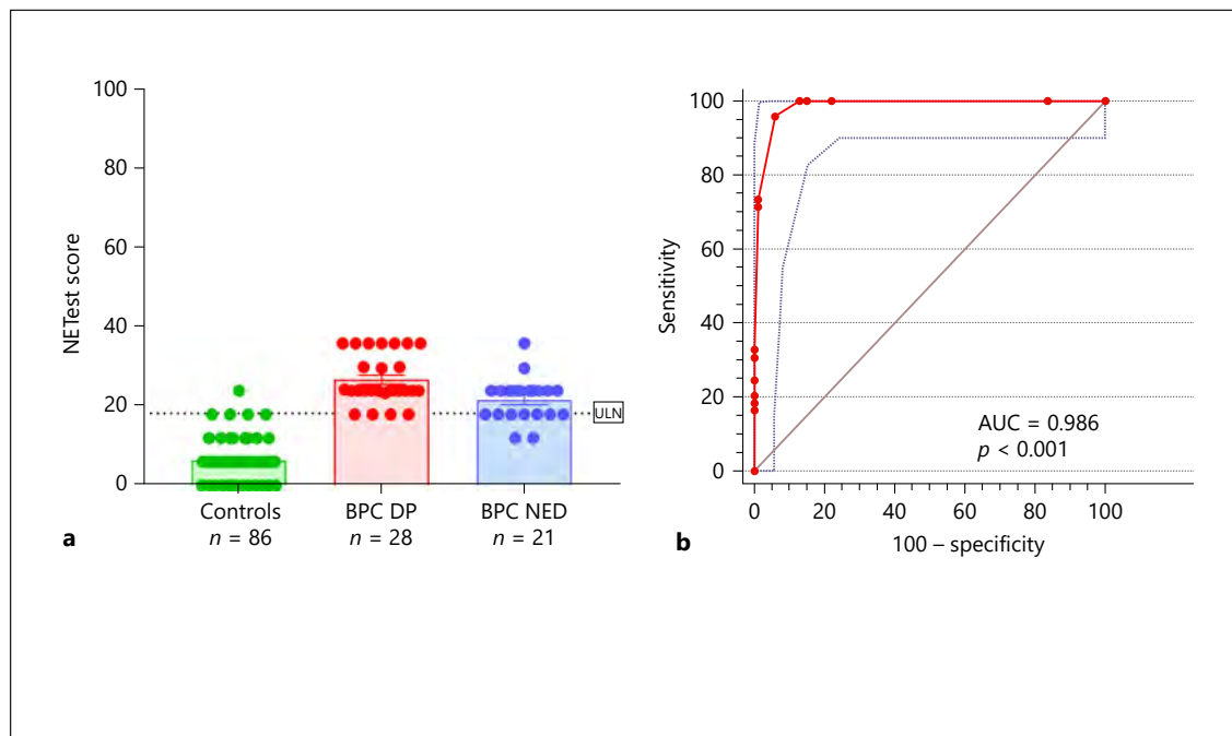
Fig. 4. NETest levels in BPC. a NETest levels in disease-positive (DP) BPC ( n = 28 ) vs. BPC with no evidence of disease (NED) and controls. KW statistic 90.3, p < 0.0001 . NETest ULN: 20%. Mean \pm SEM. b The AUROC for NETest in BPC and controls: AUC 0.99 (95% CI 0.95–0.99, p < 0.0001 ). BPC, bronchopulmonary carcinoids.
